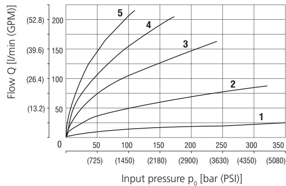
Y11/60 Nominal flow 60 l/min (15.9 GPM)
